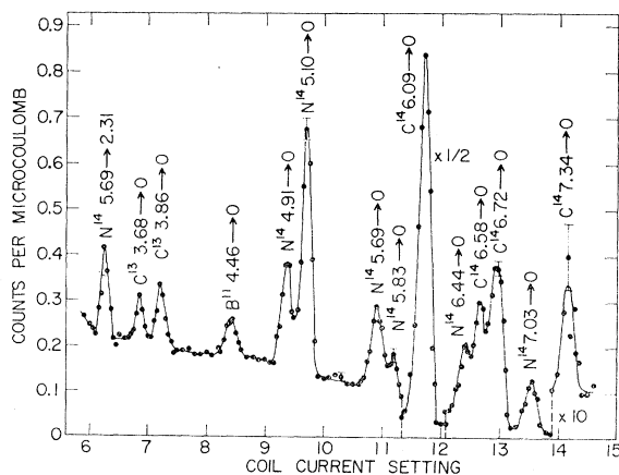
FIG. 1. Magnetic lens pair spectrum for C^{12,13}+d at E_d=2.7 MeV. The pair lines are identified by the nucleus and the energy levels (in MeV) to which they are assigned. The resolution (full width at half-maximum) for this spectrum is 2%.
